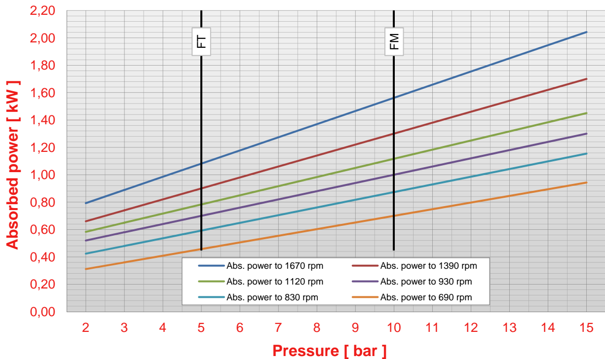
Pump F FT FM 50 pressure - abs. power chart (viscosity 50 cps)
