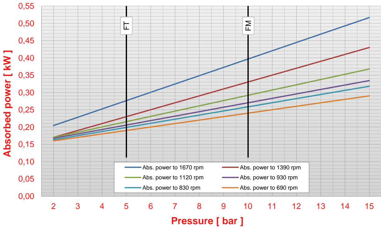
Pump F FT FM 10 pressure - abs. power chart (viscosity 50 cps)
